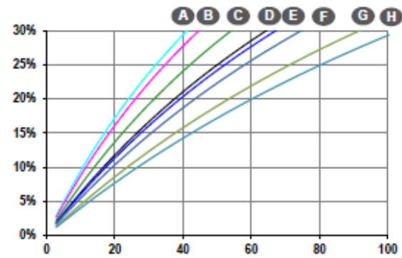
Locked rotor kVA at PF : 0.9
