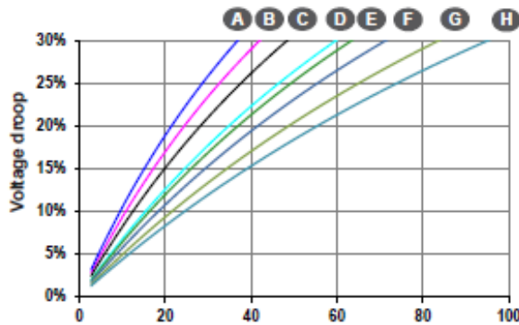
Locked rotor kVA at PF : 0.9
