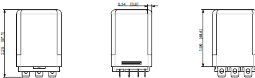
Side Flange Cover Style
