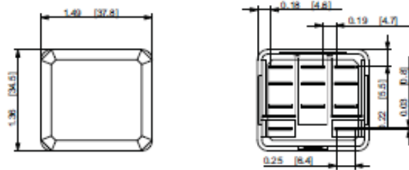
Plug-in Cover Style
